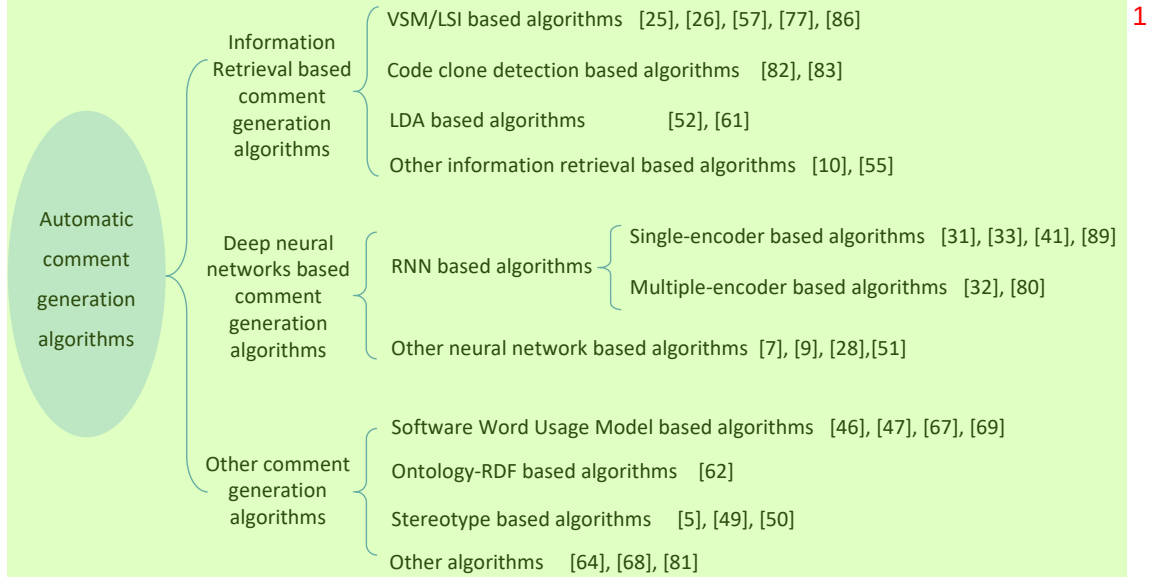
Figure 4: The classification of code comment generation algorithms and related literature.
